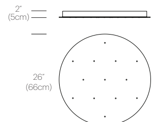
CHANDELIER CANOPY 26"
